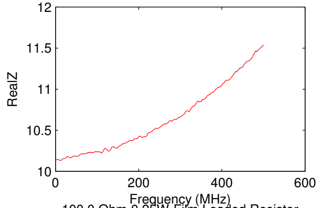
100.0 Ohm 0.25W Film Ledged Resistor
