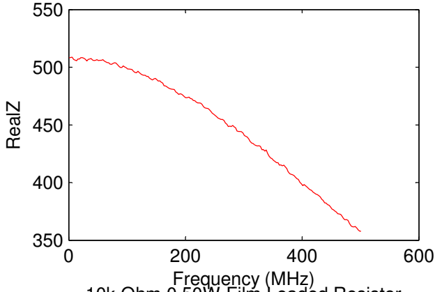
10k Ohm 0.50W Film Ledged Resistor
