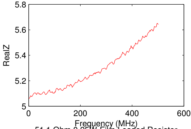
51.1 Ohm 0.25W Film Ledged Resistor
