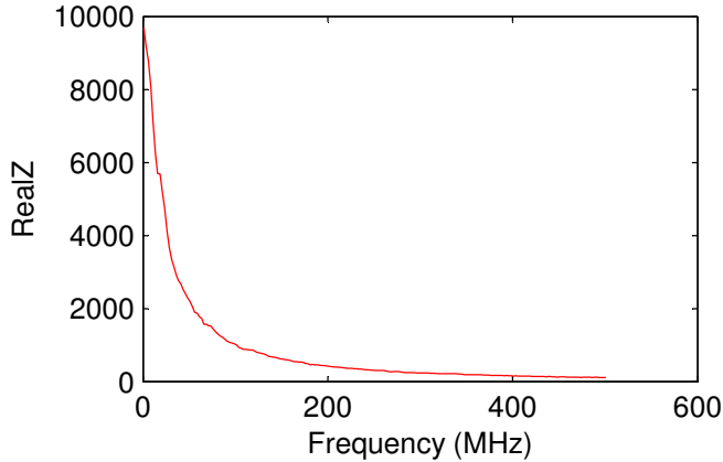
10k Ohm 0.50W Film Ledged Resistor
