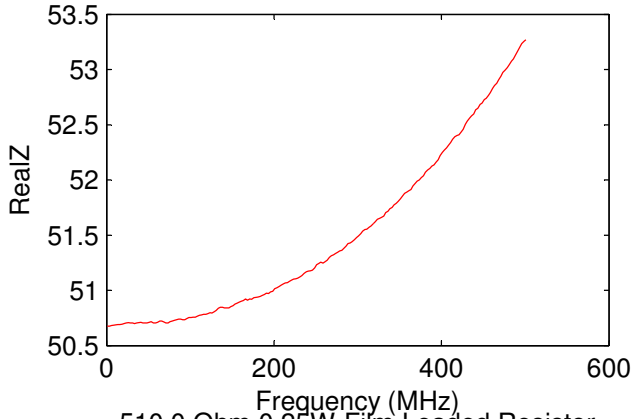
510.0 Ohm 0.25W Film Ledged Resistor
