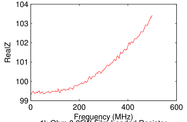
1k Ohm 0.25W Film Ledged Resistor
