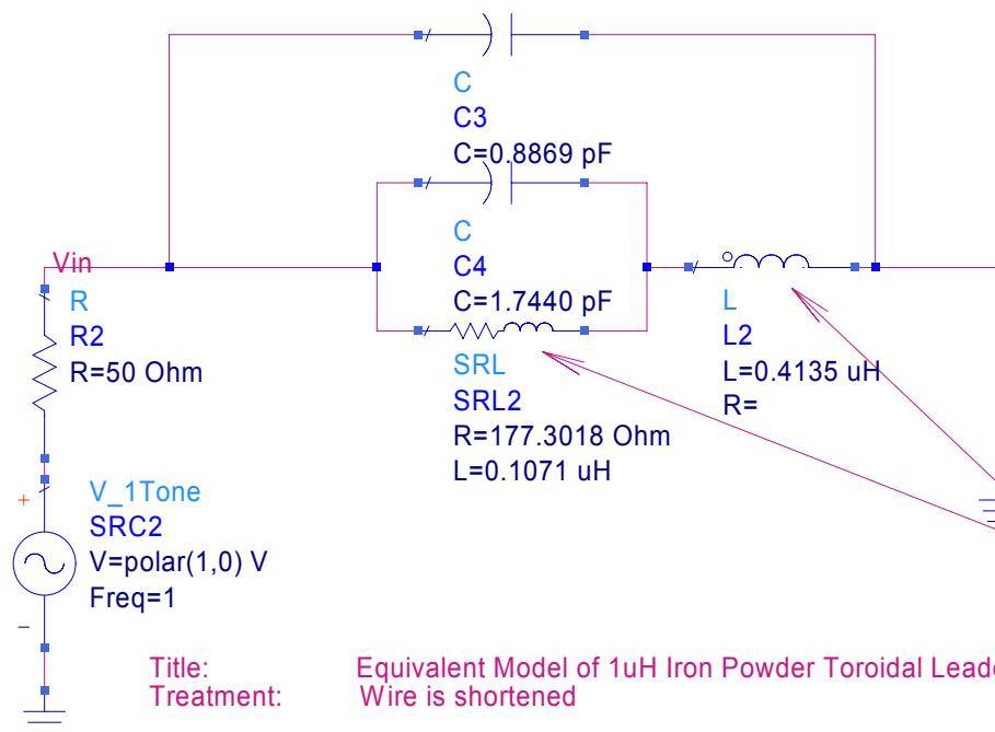
Title: Equivalent Model of 1uH Iron Powder Toroidal Leded Inductor (T-50 #3) Version #1 Treatment: Wire is shortened
