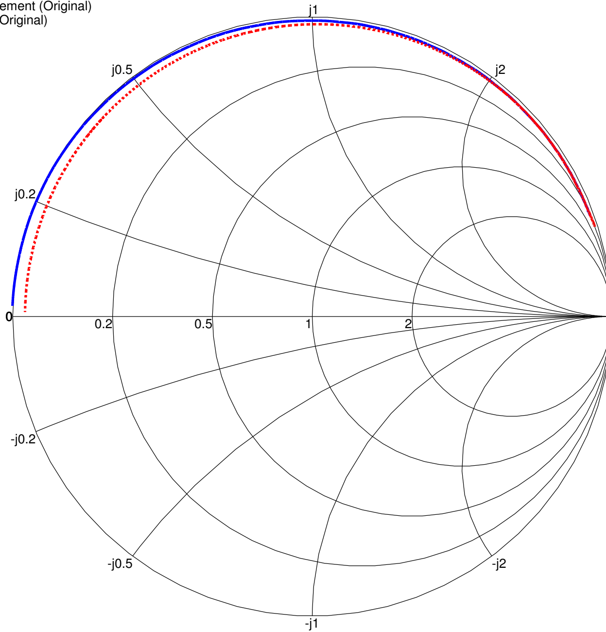
0.1uH Air-Core Leaded Inductor with Wire Shortened
