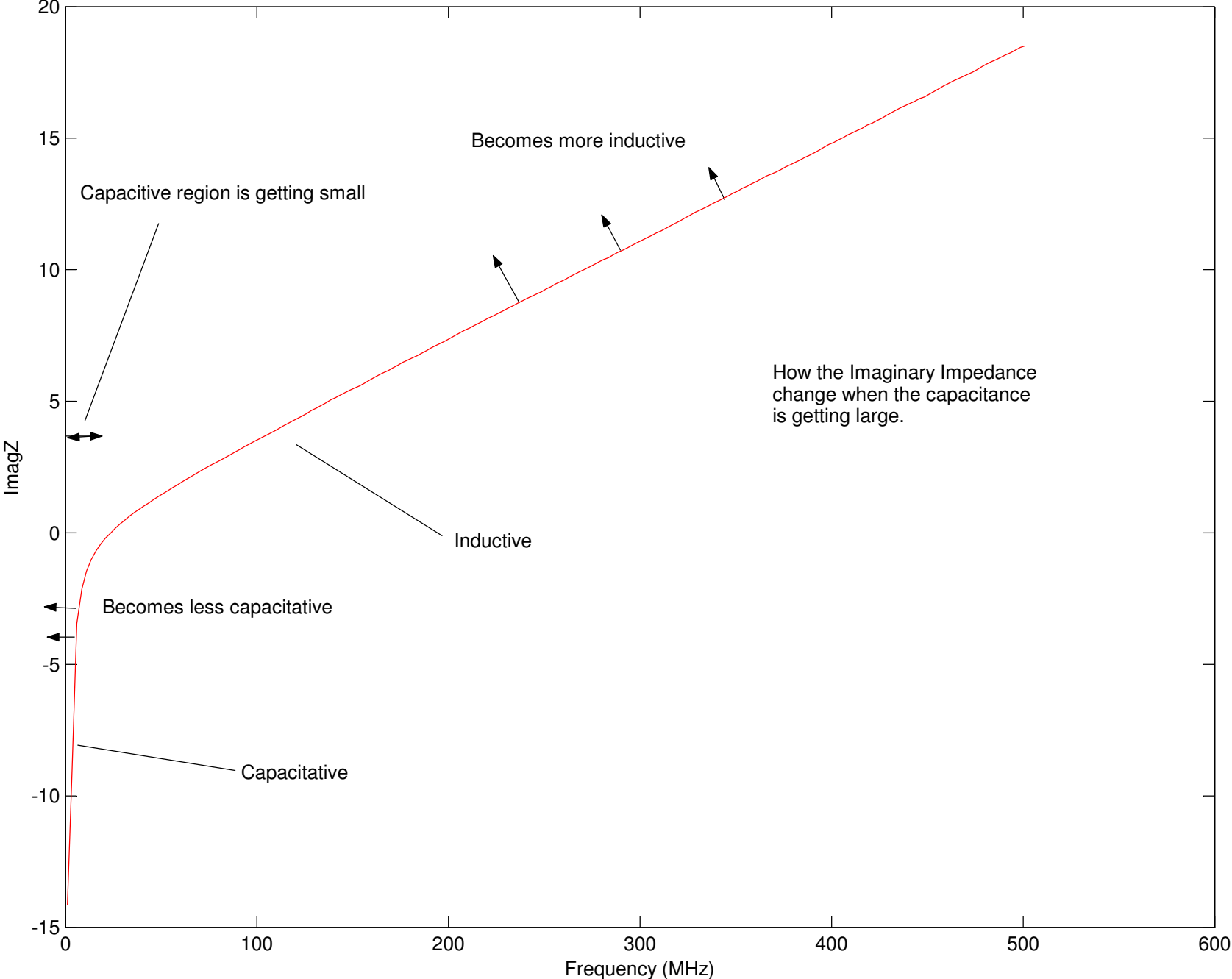
0.01 \mu F Monolithic Leaded Capacitor (Measurement, with wire shortened) Imaginary Impedance VS Frequency
