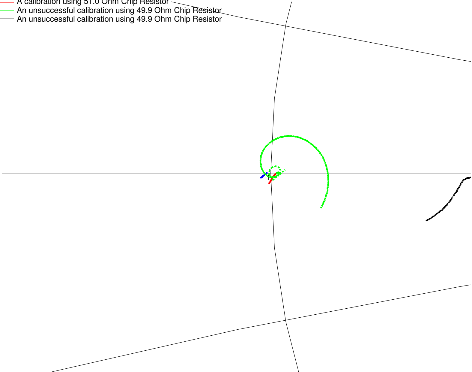
Smith Chart of Calibration Results (Zoom-In)
